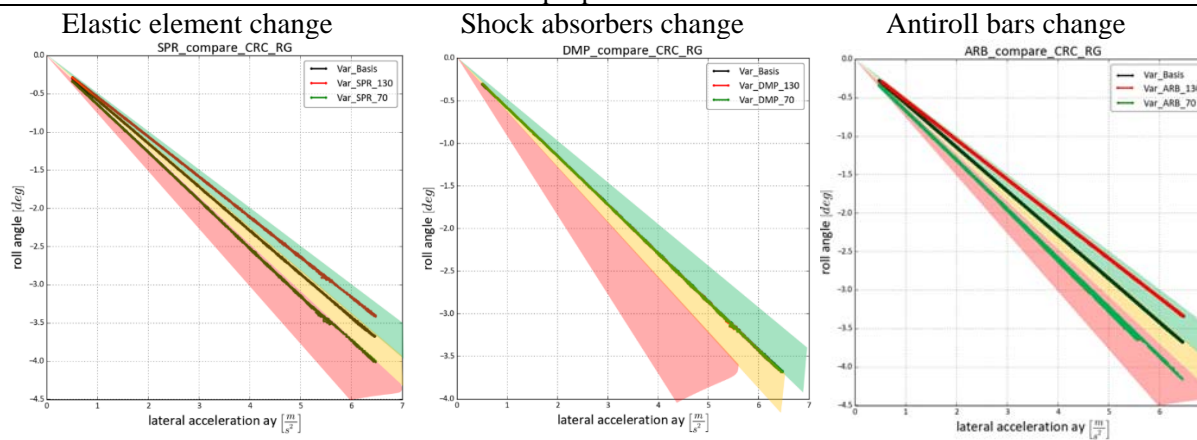
Dependence of the lateral roll angle on transverse acceleration, with change of components' properties
